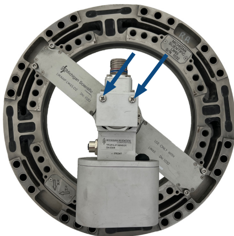
#8-32 x 9/16 in Screws
